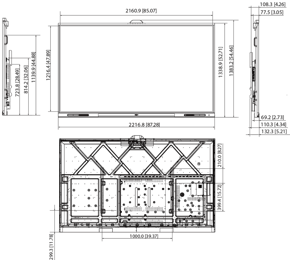
Figure 1-5 Dimensions (mm [inch])
