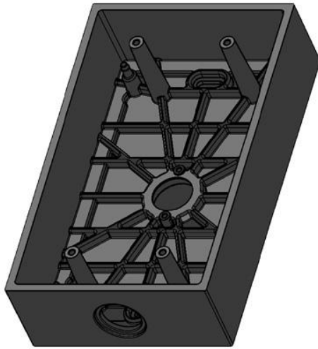
9153003 Wall mounting box (Al casting)
