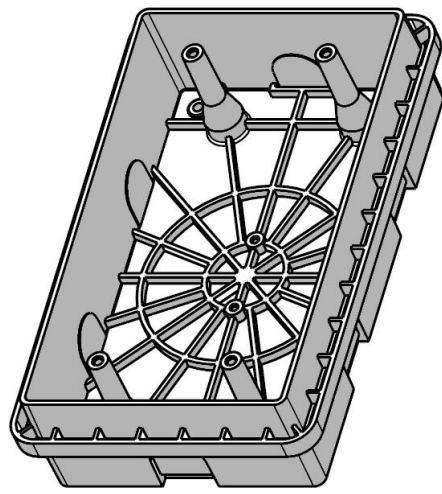
Brick flush mounting box (included in the delivery)
