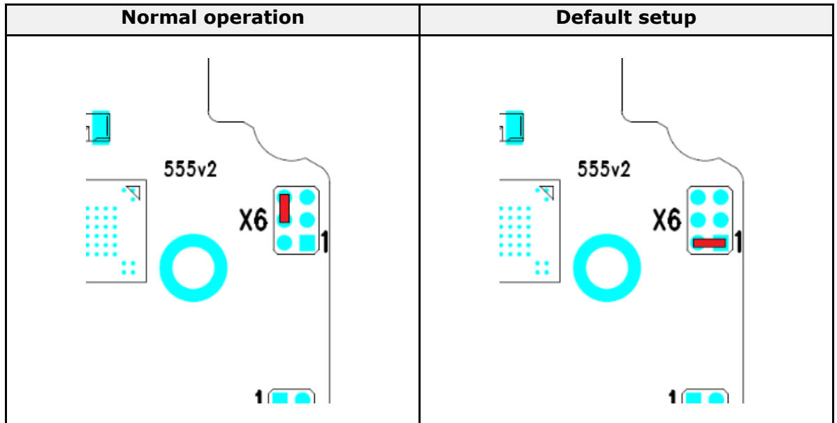
Figure: Configuration jumpers X6, PCB version 555v2
